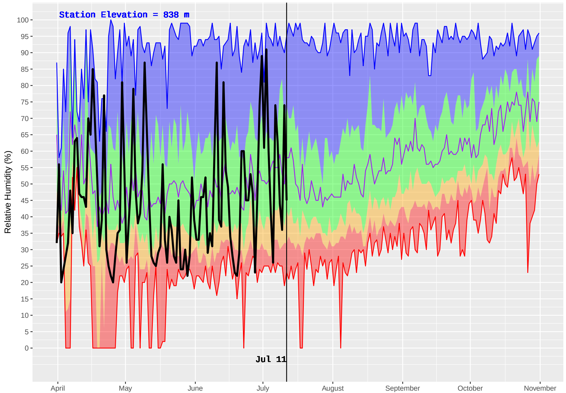
HOWARD (343) : Historical (1970–2016) and Current (2018) Noon Relative Humidity
