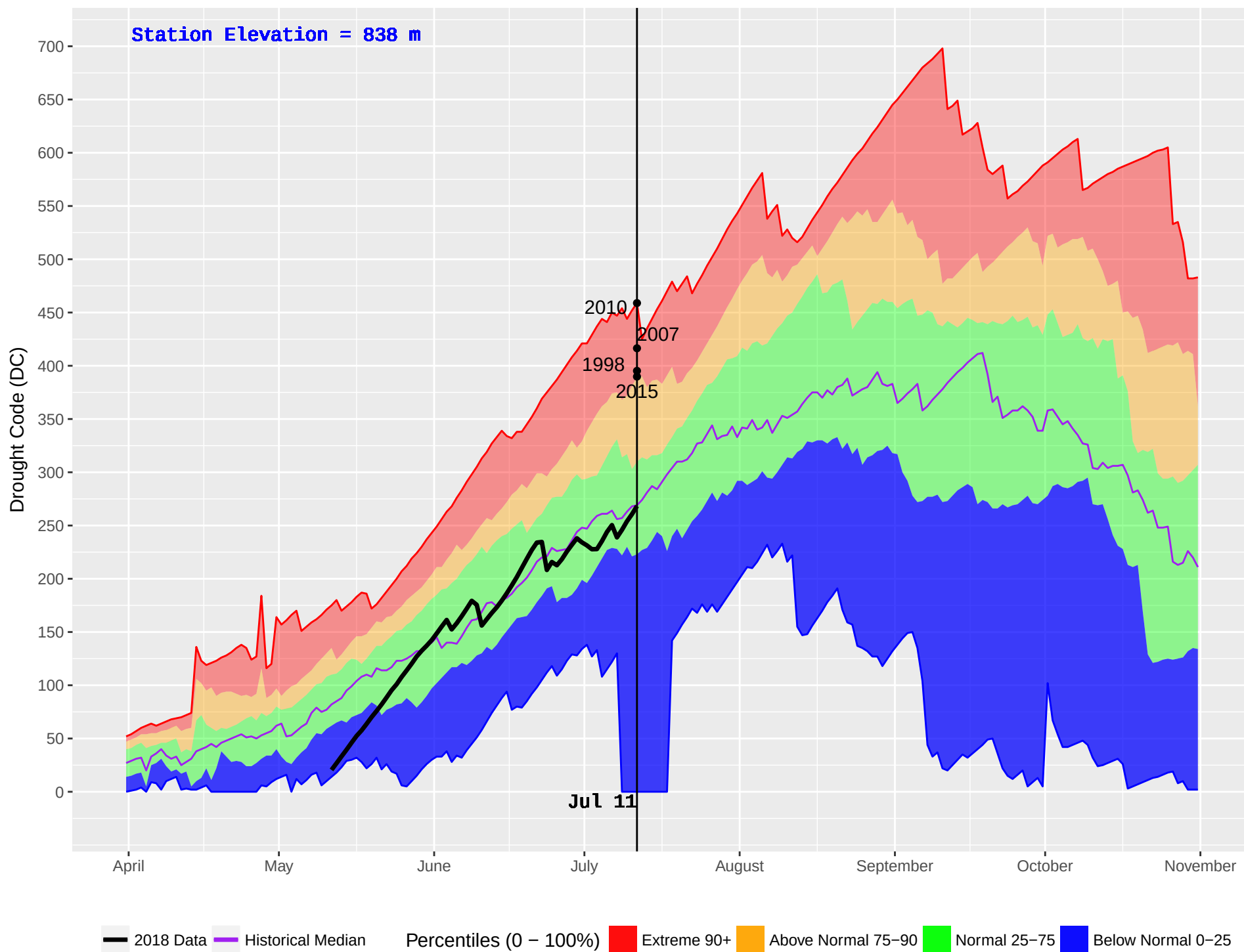
HOWARD (343) : Historical (1970–2016) and Current (2018) Noon Drought Code (DC)
