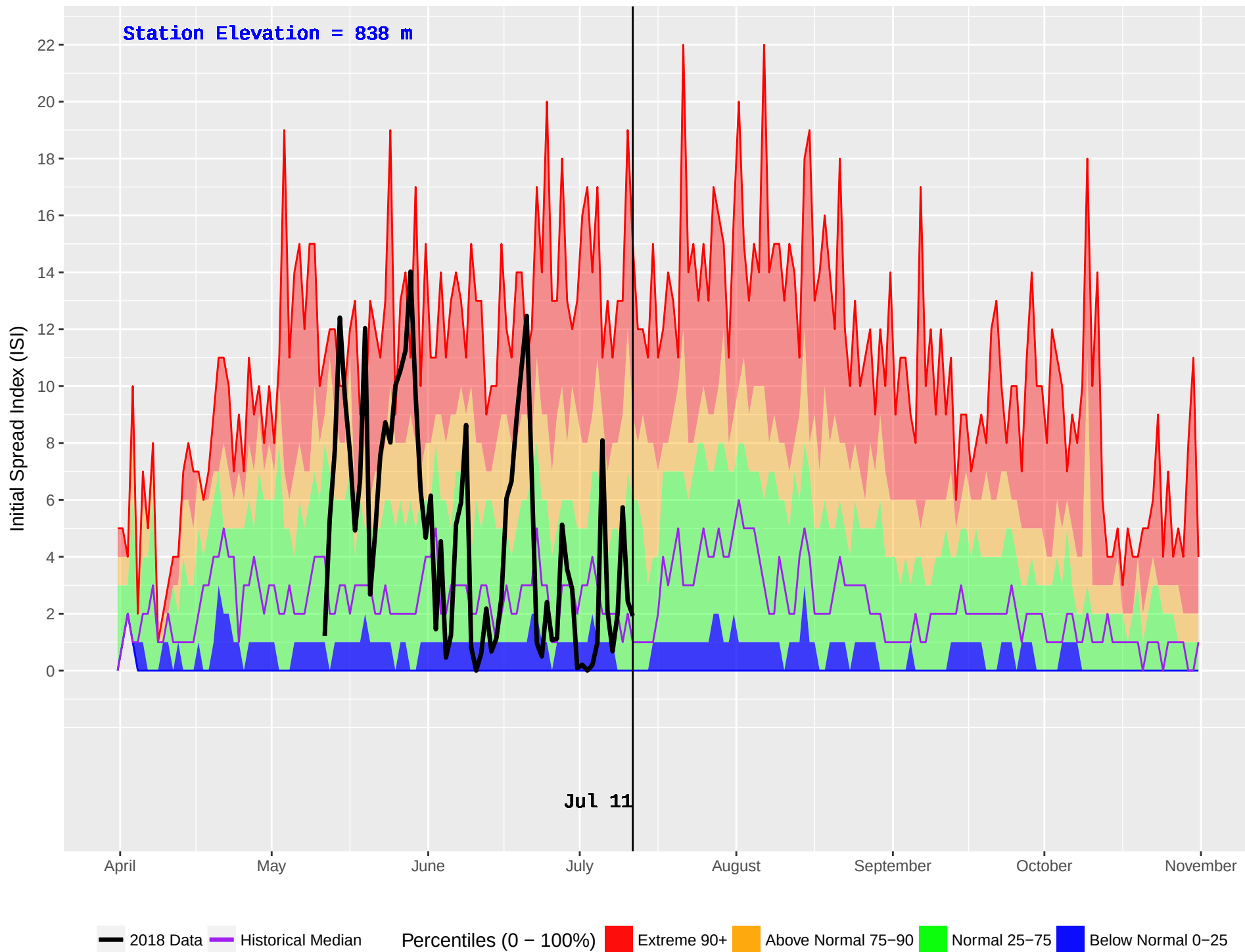
HOWARD (343) : Historical (1970–2016) and Current (2018) Noon Initial Spread Index (ISI)
