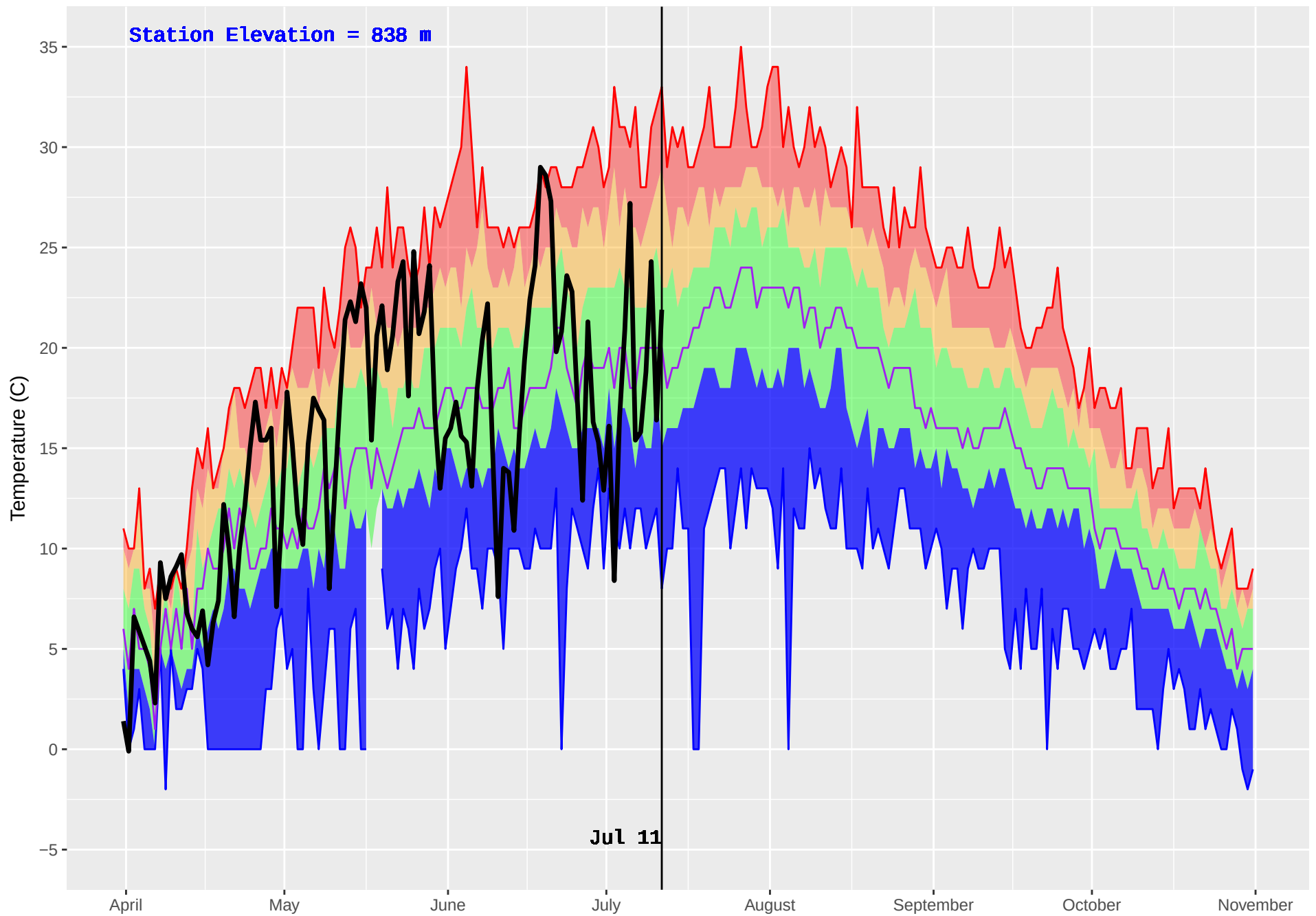
HOWARD (343) : Historical (1970–2016) and Current (2018) Noon Temperature
