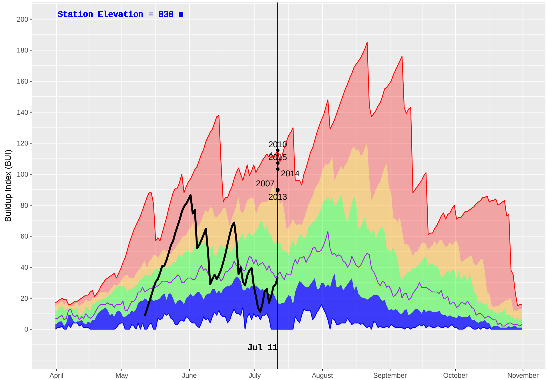
HOWARD (343) : Historical (1970–2016) and Current (2018) Noon Buildup Index (BUI)
