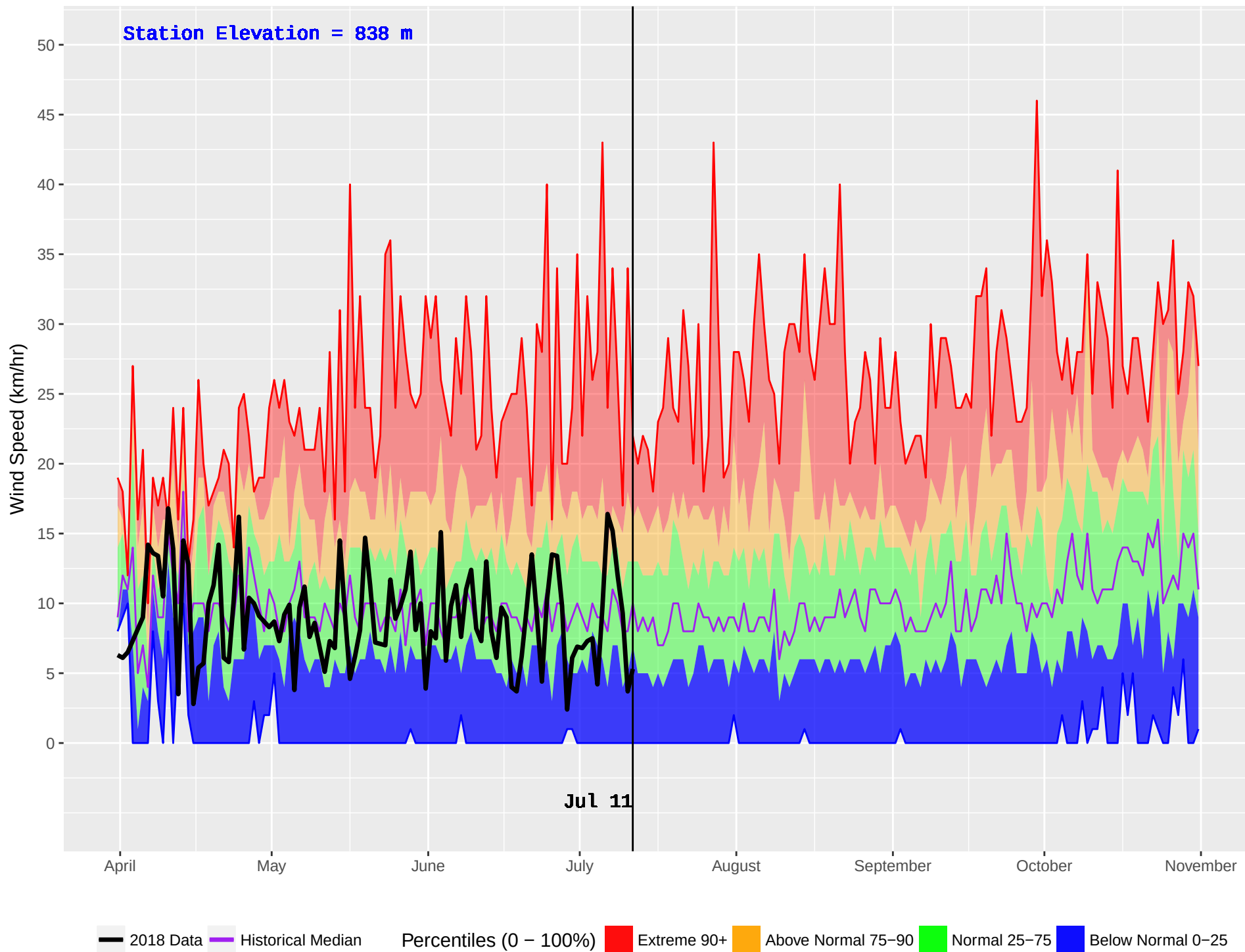
HOWARD (343) : Historical (1970–2016) and Current (2018) Noon Wind Speed
