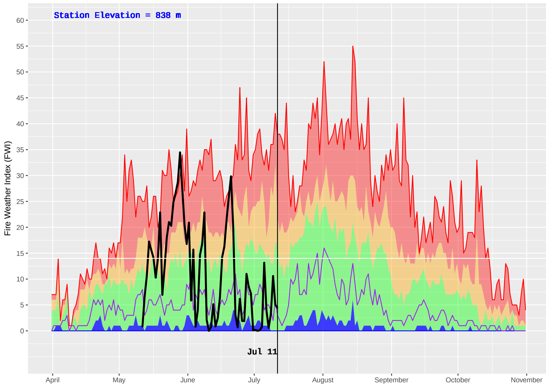
HOWARD (343) : Historical (1970–2016) and Current (2018) Noon Fire Weather Index (FWI)
